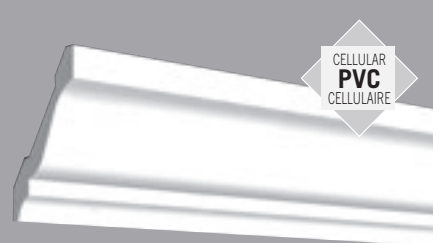
AK-AZM-47 5" Couronne / 5" Crown H: 3 5/8" P: 2 7/8" Lg: 16'
