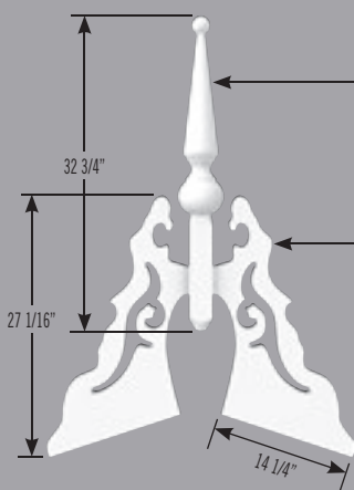
4321-P Poteau de fleuron Finial Post L/W: 4 7/8" H: 32 3/4" P: 4 7/8"
