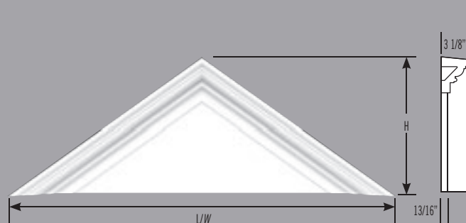
Fronton en pointe Peaked Pediment
