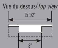
1093 Pilastre lisse en fuseau Plain Tapered Pilaster L/W: 15 1/2" H: 90" P: 4 3/8"
