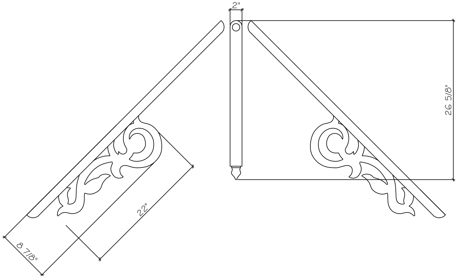
Aile de face / Wing Front View
