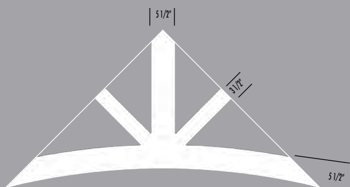
4372 Ornement de pignon courbé Curved Gable Ornament L/W: 72" H: 42" P: 1" Pente/Pitch: 8/12 à/to 14/12
