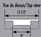
1093 Pilastre lisse en fuseau Plain Tapered Pilaster L/W: 15 1/2" H: 90" P: 4 3/8"
