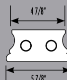
1311 Lisse Bottom Rail L/W: 5 7/8" H: 2 7/8" Lg: 144"
