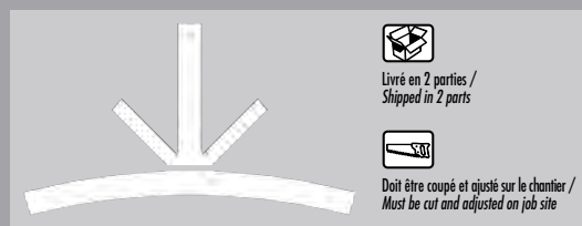
4372 Ornement de pignon courbé Curved Gable Ornament L/W: 72" H: 42" P: 1" Pente/Pitch: 8/12 à/to 14/12
