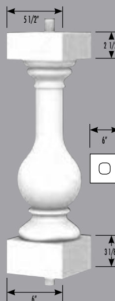
1327 Balustre Baluster L/W: 6" H: 21 7/8" P: 6" "M": 1 1/16"
