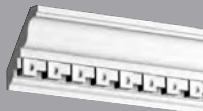
6123 Moulure dentelée Dentil Moulding H: 4 1/2" P: 3 1/4" Lg: 96" Rep: 1 3/4"
