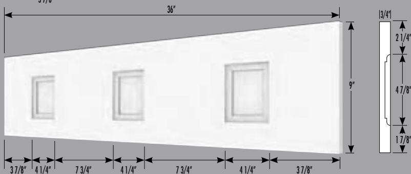
4601 Panneau de corniche Cornice Panel H: 3/4" P: 9" Lg: 36"
