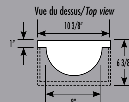
1094 Pilastre demie-colonne Half Column Pilaster L/W: 10 3/8" H: 102" P: 6 3/8"
