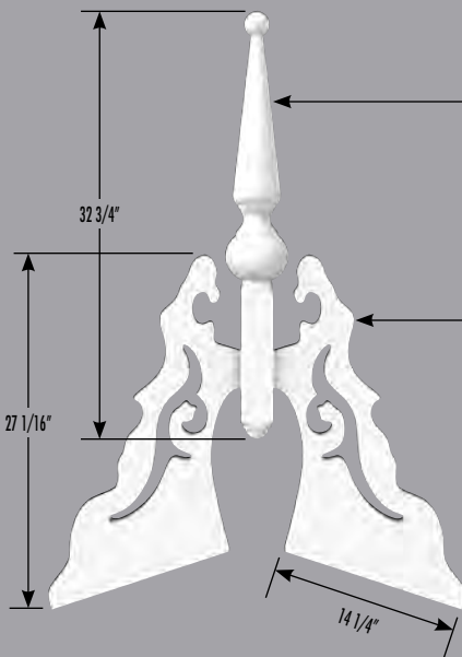
4363-P Pointe de pignon Gable Spire L/W: 7 3/4" H: 35 7/8" P: 7 3/4"
